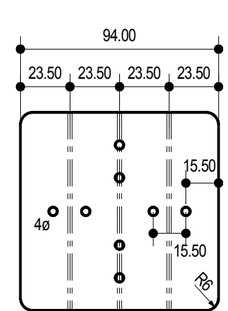
PIT 01560 / PIT 01800 Infill Panel
