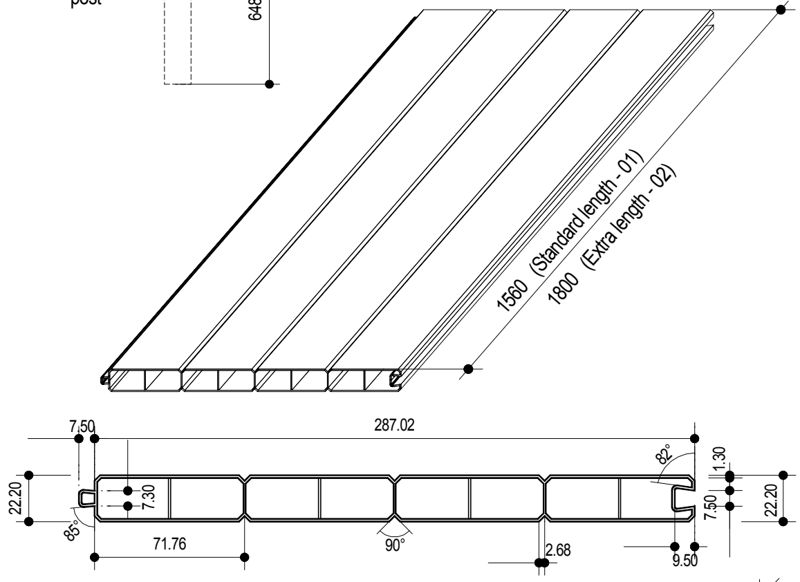
PIT 01560 / PIT 01800 Infill Panel
